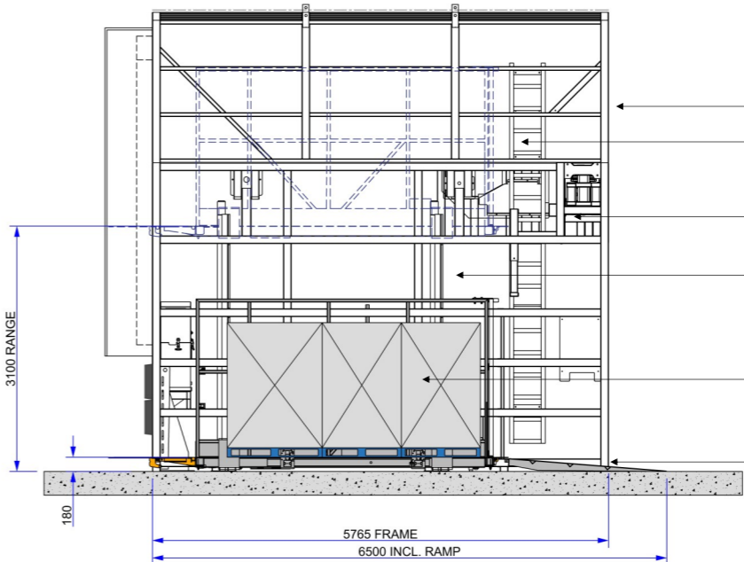
SECTION THROUGH LIFT SHOWING PLATFORM SERVICE RANGE
